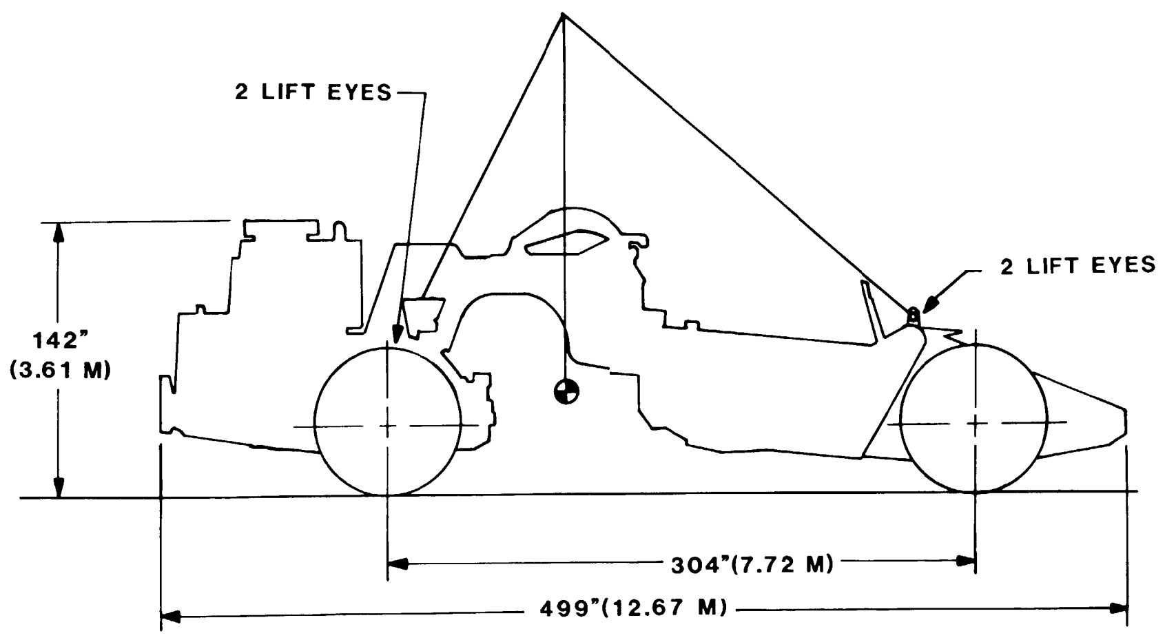
Figure 6-2: Lifting diagram for tractor-scraper.
