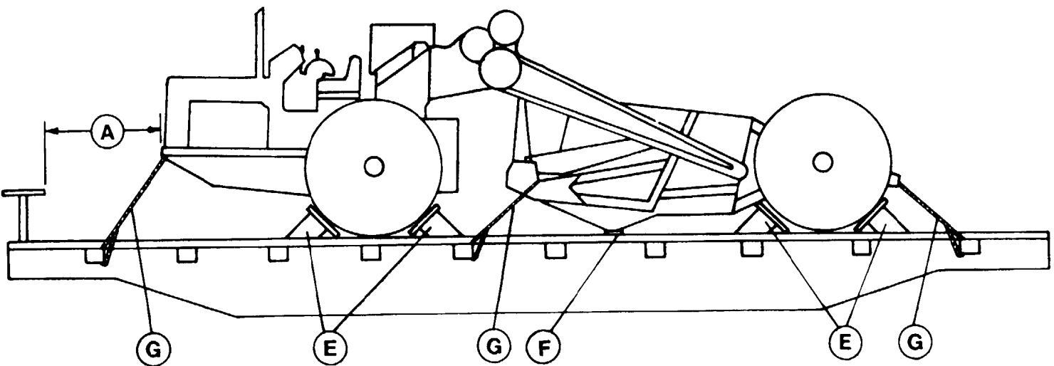
Figure 7-1. Side view of tractor-scraper loaded and restrained on a general-purpose flatcar.
