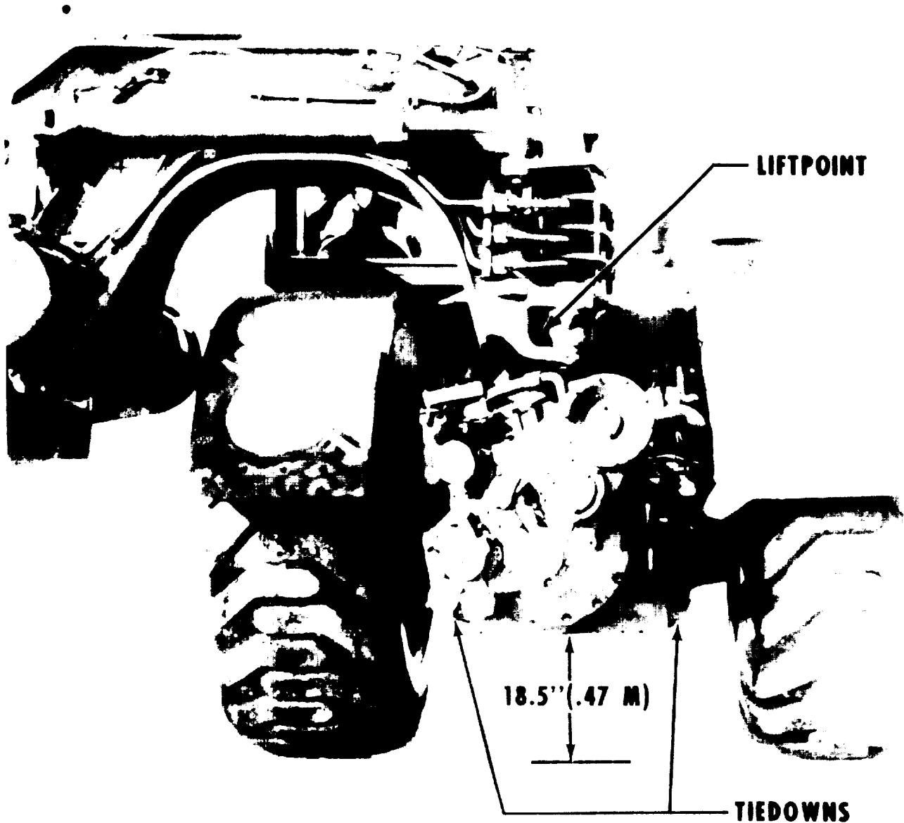
Figure 6-1. Tractor-Scraper front lift points and tiedown points
